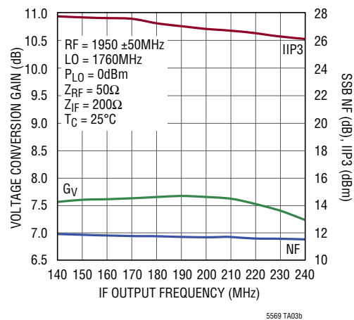
Voltage Conversion Gain, IIP3 and NF vs IF Frequency
