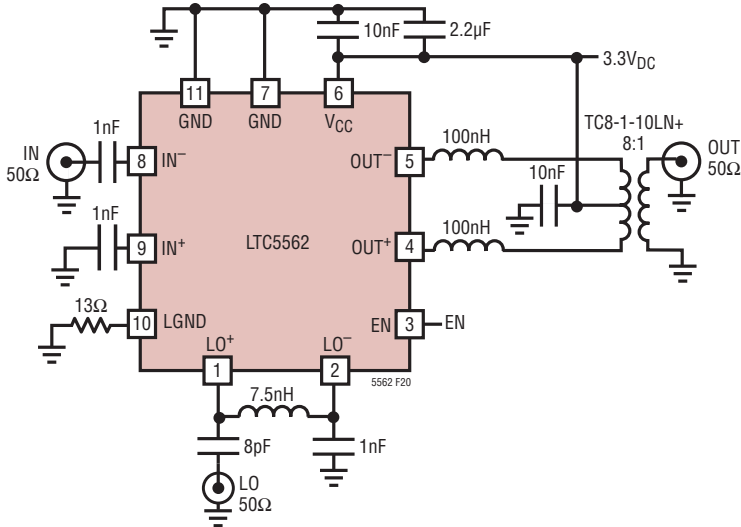
Figure 20. Low Power, Single-Ended Input, Downconverting Mixer
