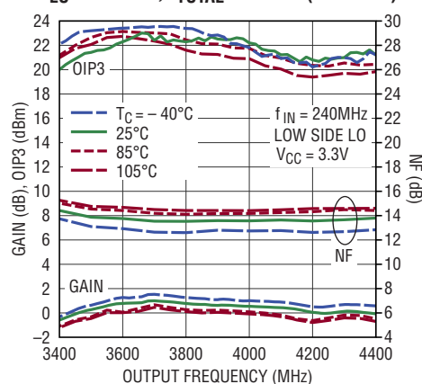
Conversion Gain, OIP3 and NF vs f_{OUT} P_{I0} = -2\text{dBm} , I_{TOTAL} = 35\text{mA} ( R1 = 5\Omega )
