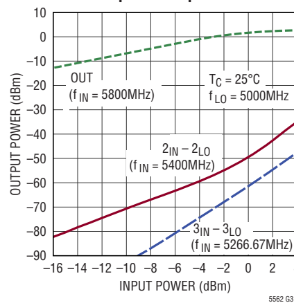
Single Tone Output Power, 2x2 and 3x3 Spurs vs Input Power
