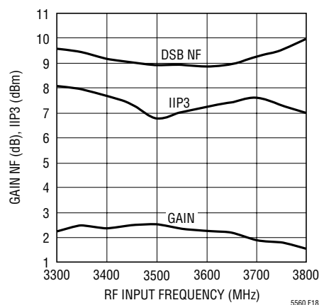
Figure 18. LT5560 Performance as a 3600MHz Downconverting Mixer
