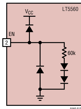
Figure 12. Enable Input Circuit
