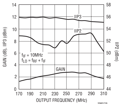
Figure 16. LT5560 Performance in 240MHz Upconverting Mixer Application
