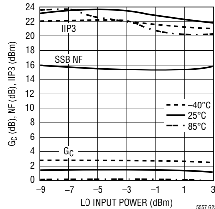
3.6GHz Conversion Gain, IIP3 and SSB NF vs LO Power
