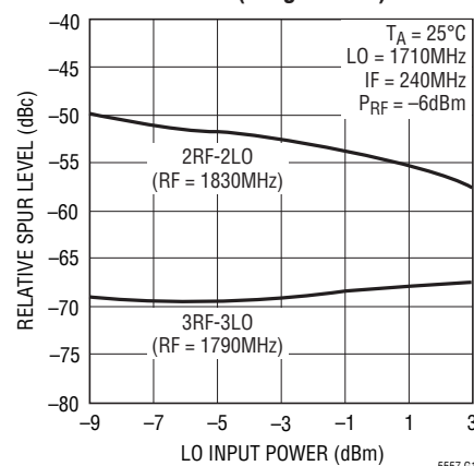
2 × 2 and 3 × 3 Spurs vs LO Power (Single Tone)
