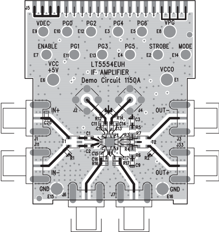
Figure 26. Silkscreen Top
