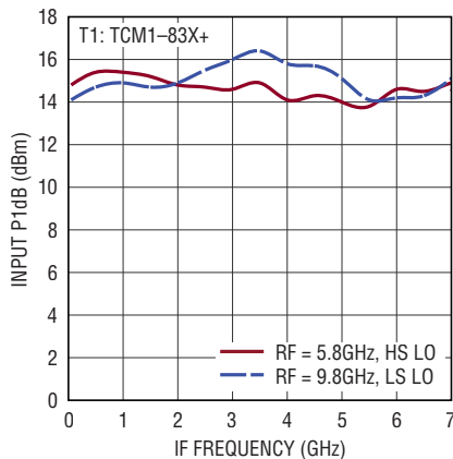
Input P1dB vs IF Frequency
