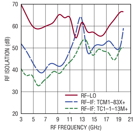
RF Isolation
