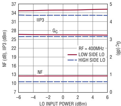
400MHz Conversion Gain, IIP3 and NF vs LO Power
