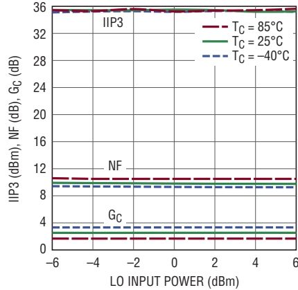
1950MHz Conversion Gain, IIP3 and NF vs LO Power (Low Side LO)
