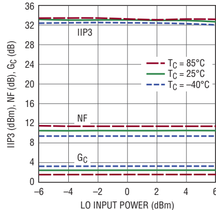
1950MHz Conversion Gain, IIP3 and NF vs LO Power (High Side LO)
