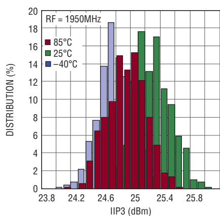
IIP3 Distribution
