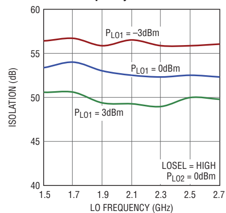
LO Switch Isolation vs LO Frequency—LO2 Selected
