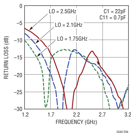
Figure 4. RF Input Return Loss
