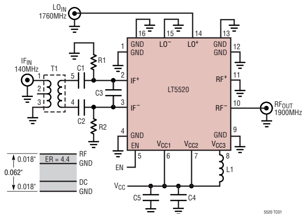
Figure 2. Test Schematic for the LT5520
