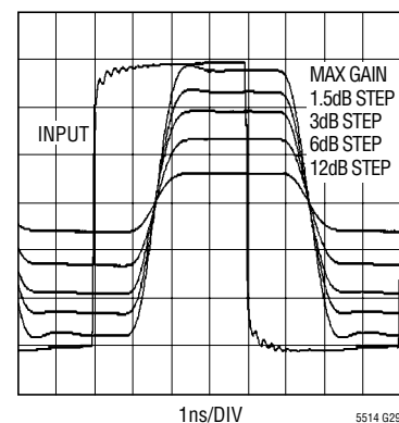
Pulse Response vs Attenuation, Output Level is 2V_{P-P} at Max Gain into 50\Omega External Load
