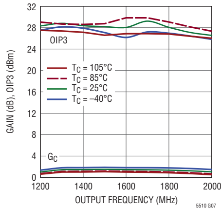
Conversion Gain and OIP3 vs Output Frequency
