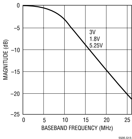
LPF Frequency Response vs Baseband Frequency and Supply Voltage
