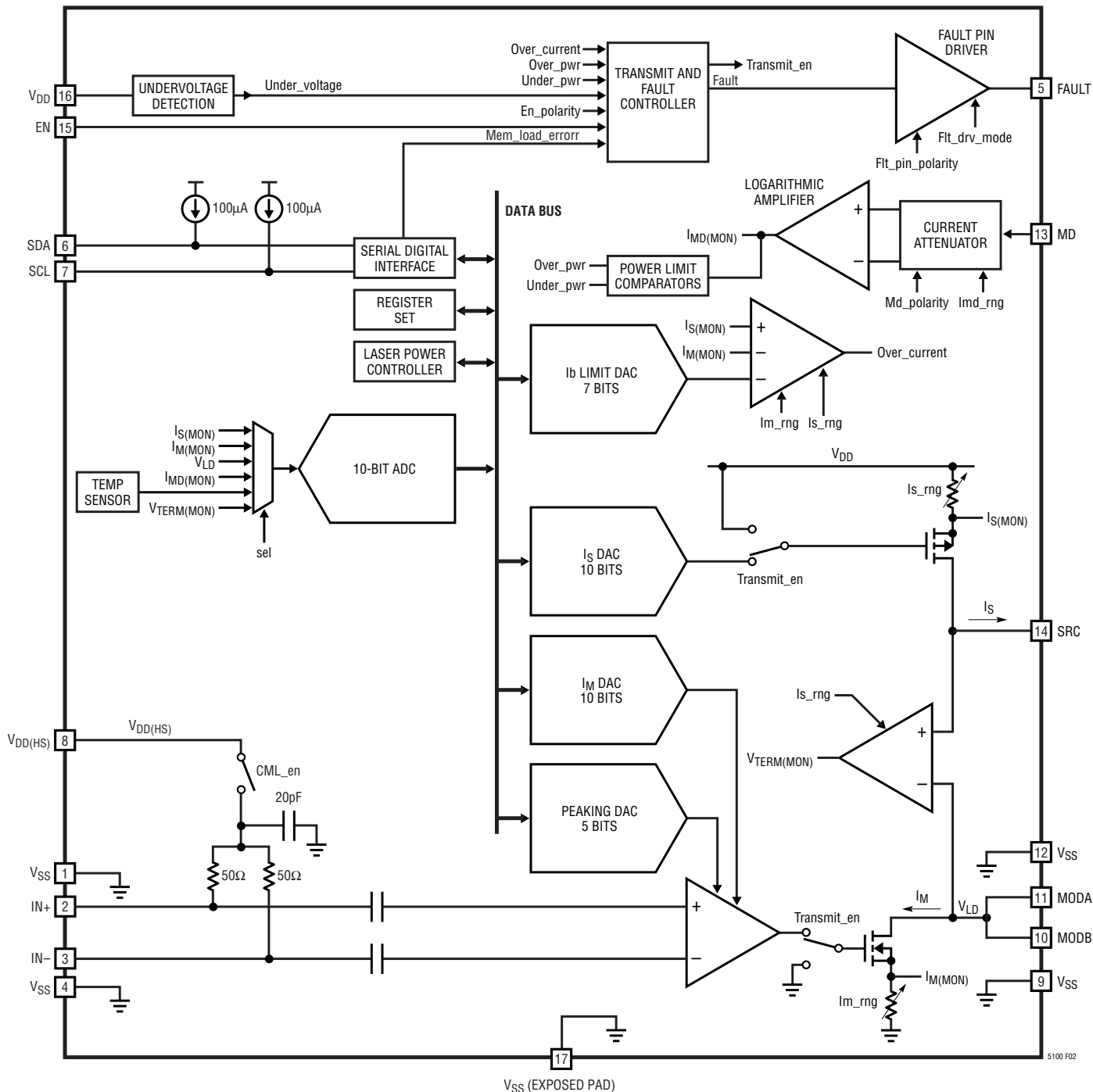
Figure 2. Block Diagram
