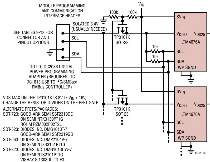
Figure 5. Circuit Suitable for Programming EEPROM/NVM of LTM4676A and Other ADI PSM Modules/ICs in Vast Systems, Even When V IN Power is Absent, 0°C < T J ≤ 85°C
