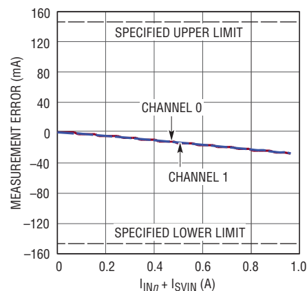
MFR_READ_IIN n (Input Current Readback) Error vs (I_{\text{VIN}n} + I_{\text{SVIN}}) , \text{MFR\_PWM\_MODE}_n[0]=1_b , I_{\text{OUT}n} Swept from 0A to 9A, One Channel at a Time, \text{RUN}_{1-n} = 0\text{V}
