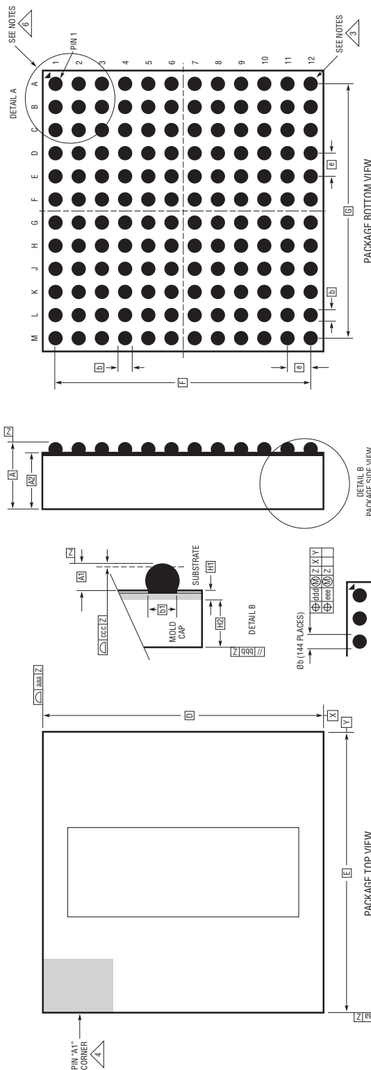
BGA Package 144-Lead (16mm × 16mm × 5.01mm) (Reference LIT DWG # 05-08-1523 Rev A)
