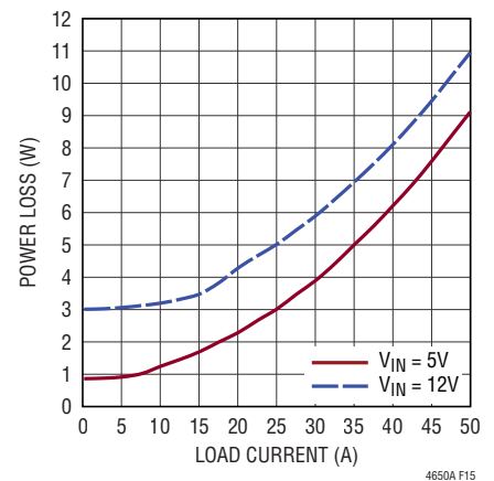
Figure 15. 3.3V OUT Power Loss Curve
