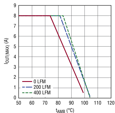
Figure 19. 20V IN , 2.5V OUT 1MHz, No Heat Sink
