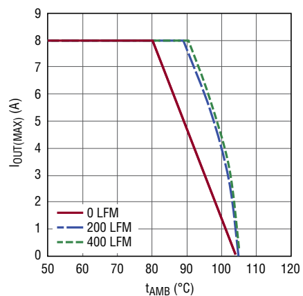
Figure 22. 12V IN , 5V OUT 1.2MHz, with Heat Sink
