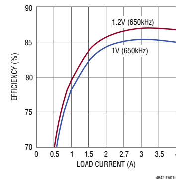
Efficiency vs Load Current at 12V input
