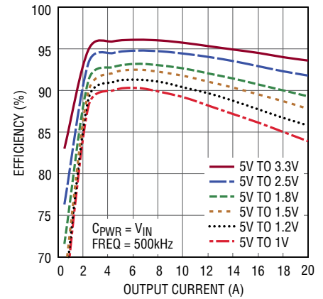
5V Efficiency Graph
