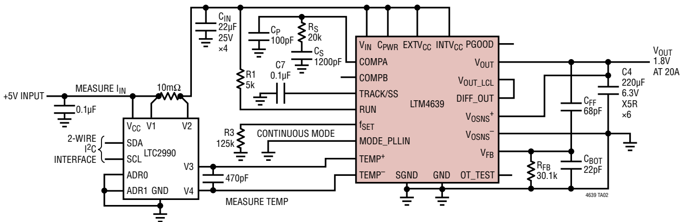
1.8V at 20A Design with Input Current and Temperature Monitoring
