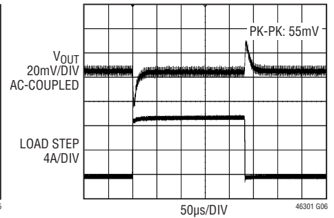
Dual Phase Single Output 25% (9A) Transient Response at 1V Output
