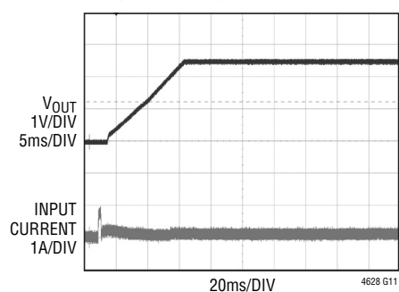
Output Start-Up
