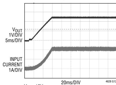
Output Start-Up
