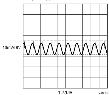
Output Ripple
