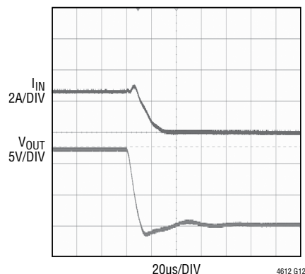
Short-Circuit with 24V_{IN} to 12V_{OUT} at I_{OUT} = 5A
