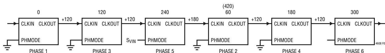
Figure 2. 6-Phase Operation
