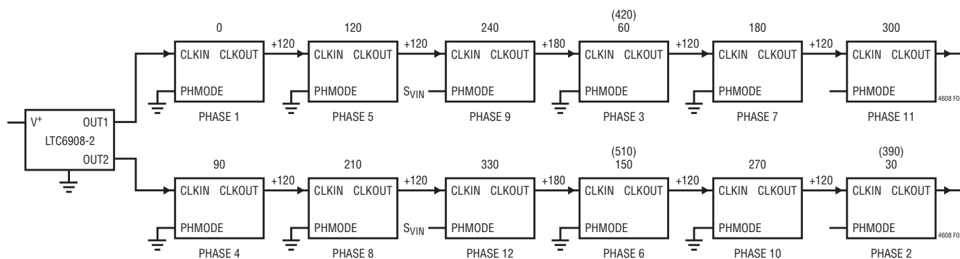
Figure 3. 12-Phase Operation
