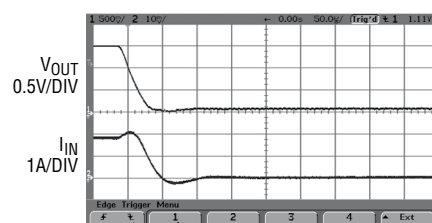
Short-Circuit Protection, I_{OUT} = 12\text{A}
