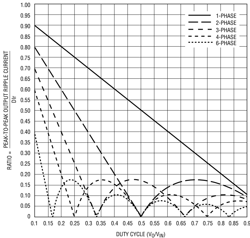
Figure 4. Normalized Output Ripple Current vs Duty Cycle, D_{Ir} = V_O T / L I_L , D_{Ir} = Each Phase's Inductor Current
