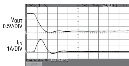
Short-Circuit Protection, I_{OUT} = 0\text{A}
