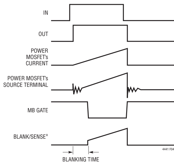
Figure 4. Blanking Waveforms
