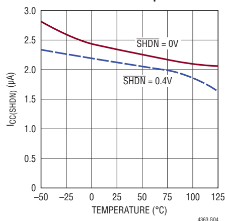
SHDN Current vs Temperature
