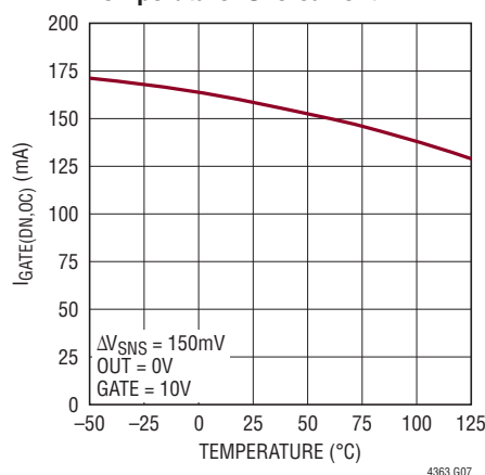
GATE Pull-Down Current vs Temperature: Overcurrent
