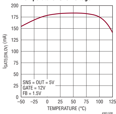
GATE Pull-Down Current vs Temperature: Overvoltage
