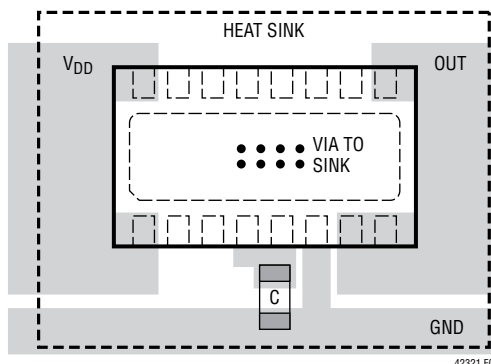
Figure 7. Recommended Layout
