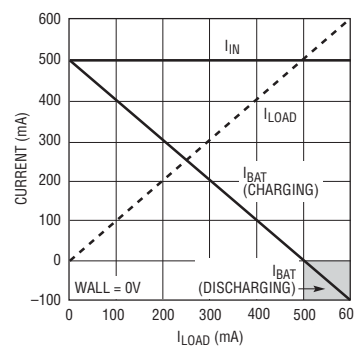
Input and Battery Current vs Load Current R PROG = 100k, R CLPROG = 2k
