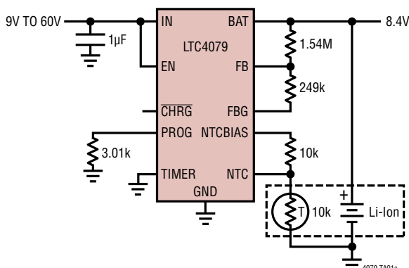
Charging a Backup Battery
