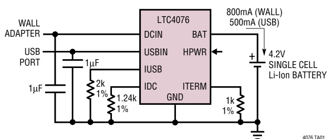
Dual Input Battery Charger for Single-Cell Li-Ion
