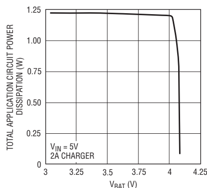
Power Loss vs V_{BAT} Charging (PWM Mode)
