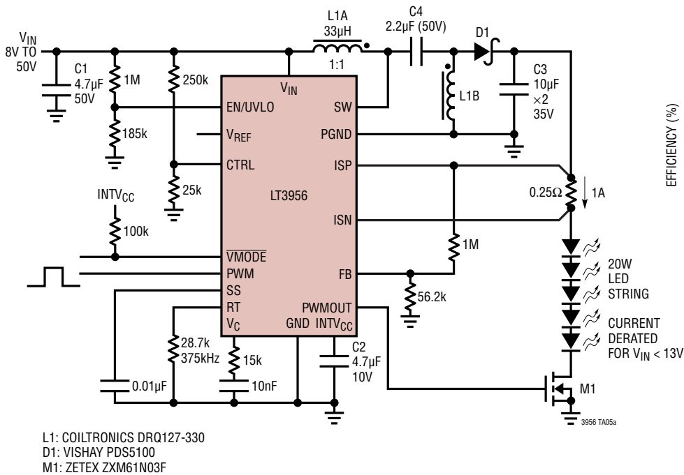
90% Efficient, 20W SEPIC LED Driver
