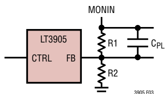
Figure 3. Phase Lead Capacitor
