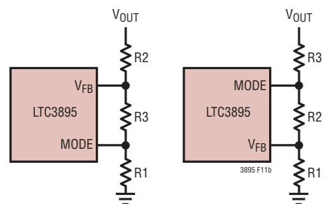
(11b) Using V FB to Program the Burst Clamp
