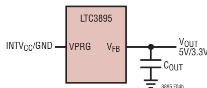
(4b) Setting Output to Fixed 5V/3.3V Voltage
