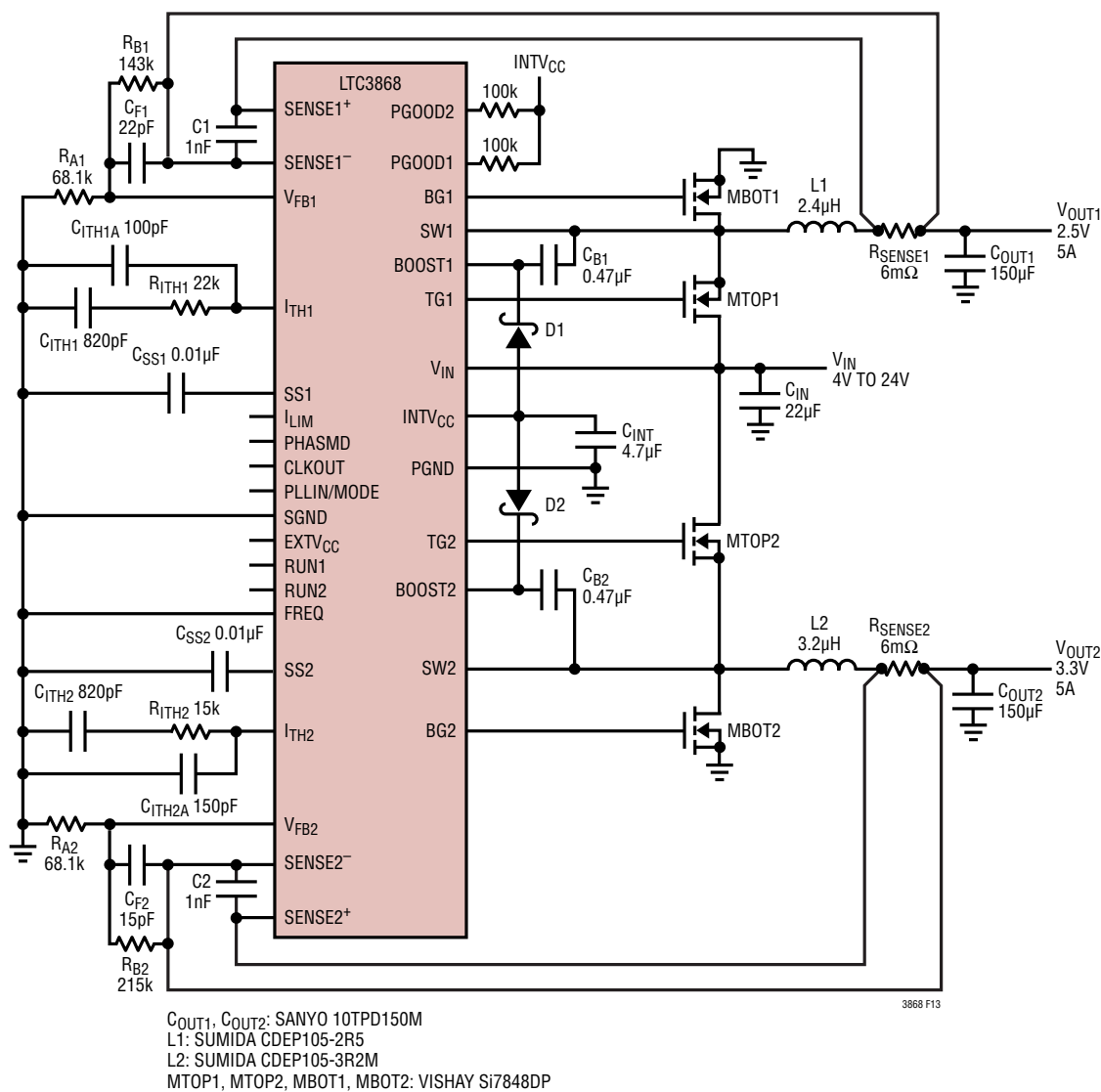
High Efficiency Dual 2.5V/3.3V Step-Down Converter
