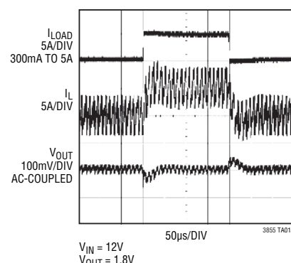
Load Step (Forced Continuous Mode)
