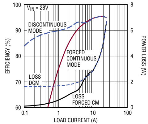
Figure 19. 6.5V to 34V Input, 5V/25A Output, 300kHz, R_{SENSE} , 5V Output Tied to EXTVC, Step-Down Converter
