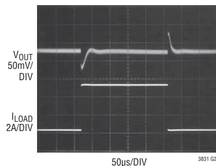
Transient Response
