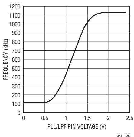
Figure 21. Relationship Between Oscillator Frequency and Voltage at the PLL/LPF Pin When Synchronizing to an External Clock
