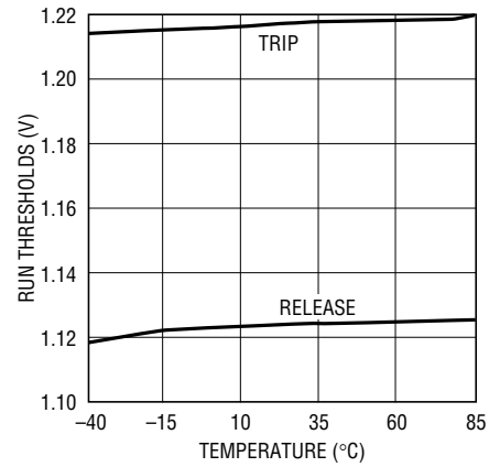
RUN Thresholds vs Temperature
