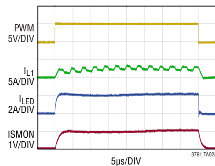
100Hz 250:1 PWM Dimming ( V_{IN} = 24V )
