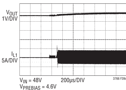
Pre-Biased Start-Up
