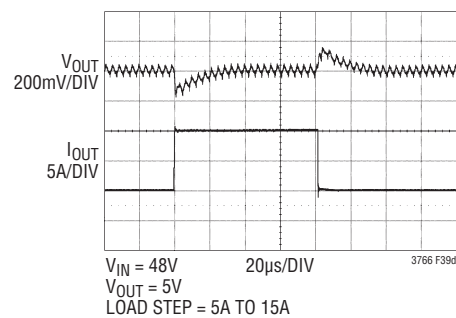
Load Step
