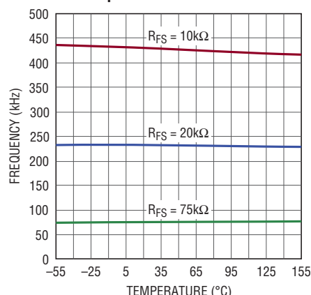
Start-Up Oscillator Frequency vs Temperature
