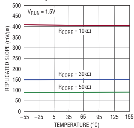
I SMAG Replicated Slope vs Temperature
