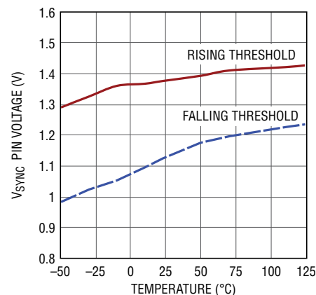
SYNC Threshold
