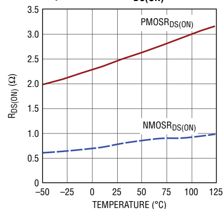
Top Gate Driver R_{DS(ON)}
