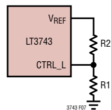
Figure 7. Analog Control of LED Current
