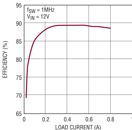
Efficiency, V_{\text{OUT}} = 5\text{V}
