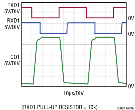
Operating Waveforms
