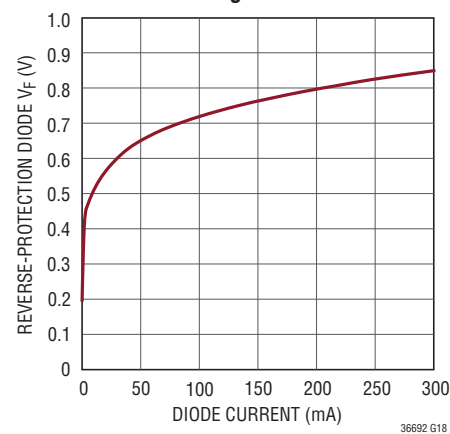
Reverse-Protection Diode Forward Voltage
