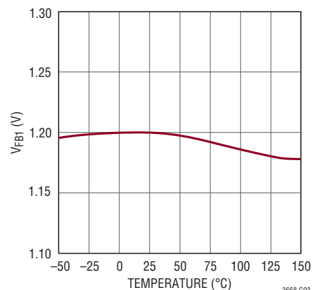
V_{FB1} vs Temperature
