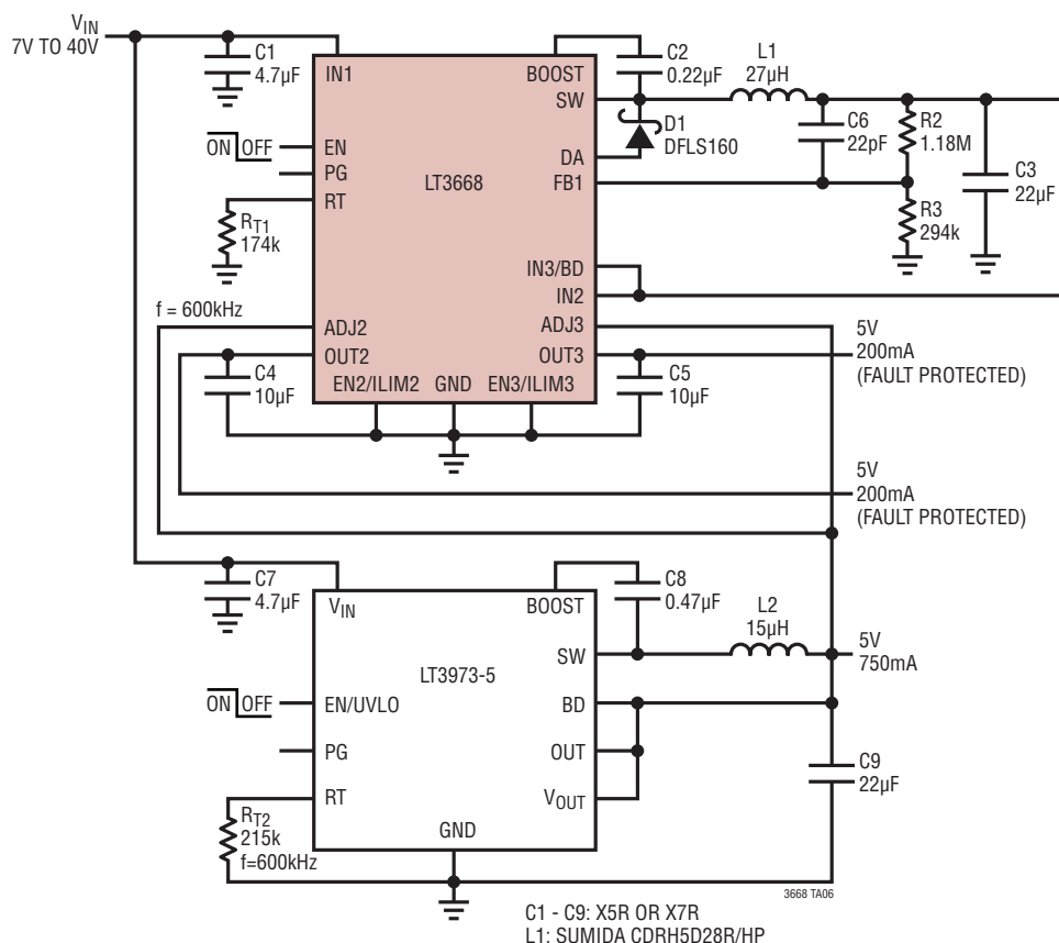
5V/0.75A Supply with Two 0.2A Tracking Outputs
