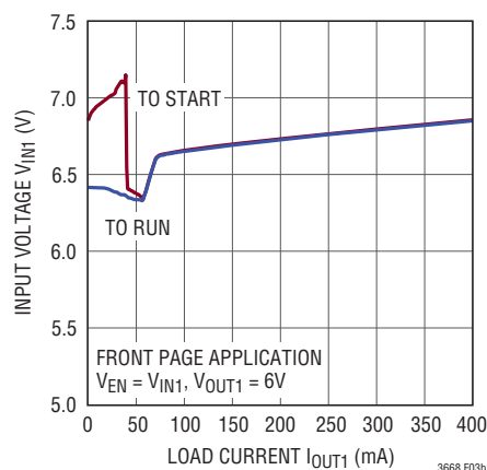
Figure 3. The Minimum Input Voltage Depends on Output Voltage, Load Current and Boost Circuit
