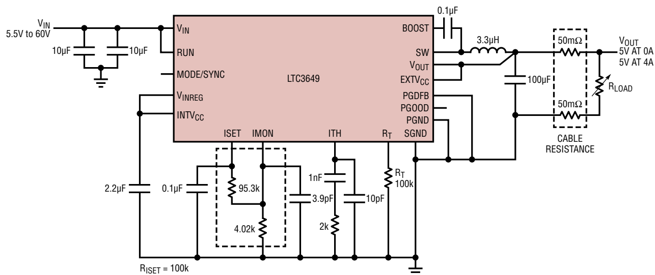
Cable Drop Compensation
