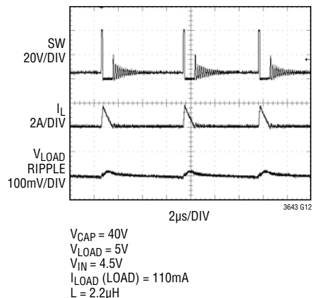
Step-Down Regulator Light Load Switching Waveform
